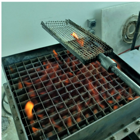
Fig. 3 A photo of the open flame burner used to conduct ignition and consumption tests. Branchwood segments were held over the flames in a wire basket while time to ignition was measured
